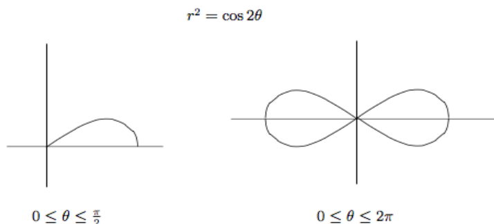
Figure 1: lemniscate
